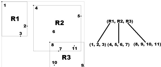
Figure 2: R-Tree Sample
